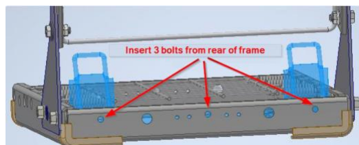
Figure 4-Bracket (blue) in install location.
